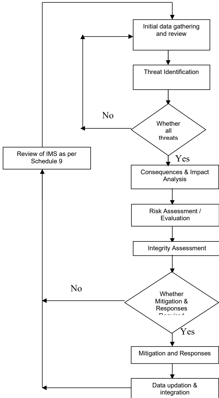
Figure-1: CGD Network Integrity Management Plan - Flow Diagram
